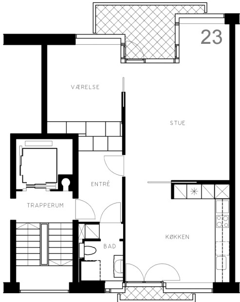
STRANDBOULEVARDEN 76-88C, 1.-3. th. TYPE 2V.4 th. - 85,1 m 2 - 27 stk.
